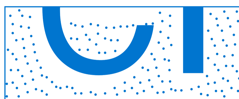
Floyd-Steinberg
